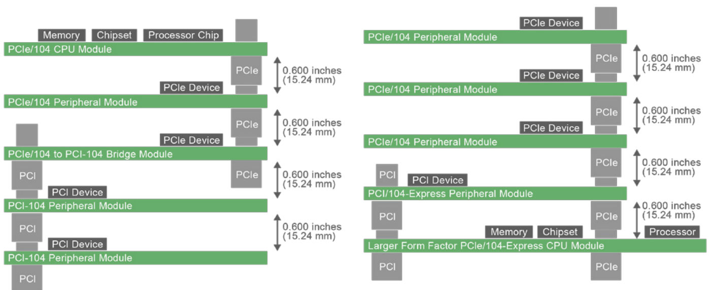
(Figure 1. PC/104 Board Stack Assembly)
