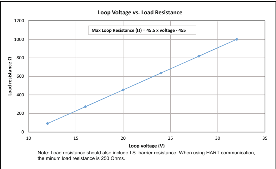
Figure 2-2 Power Supply vs. Maximum Load Resistance
