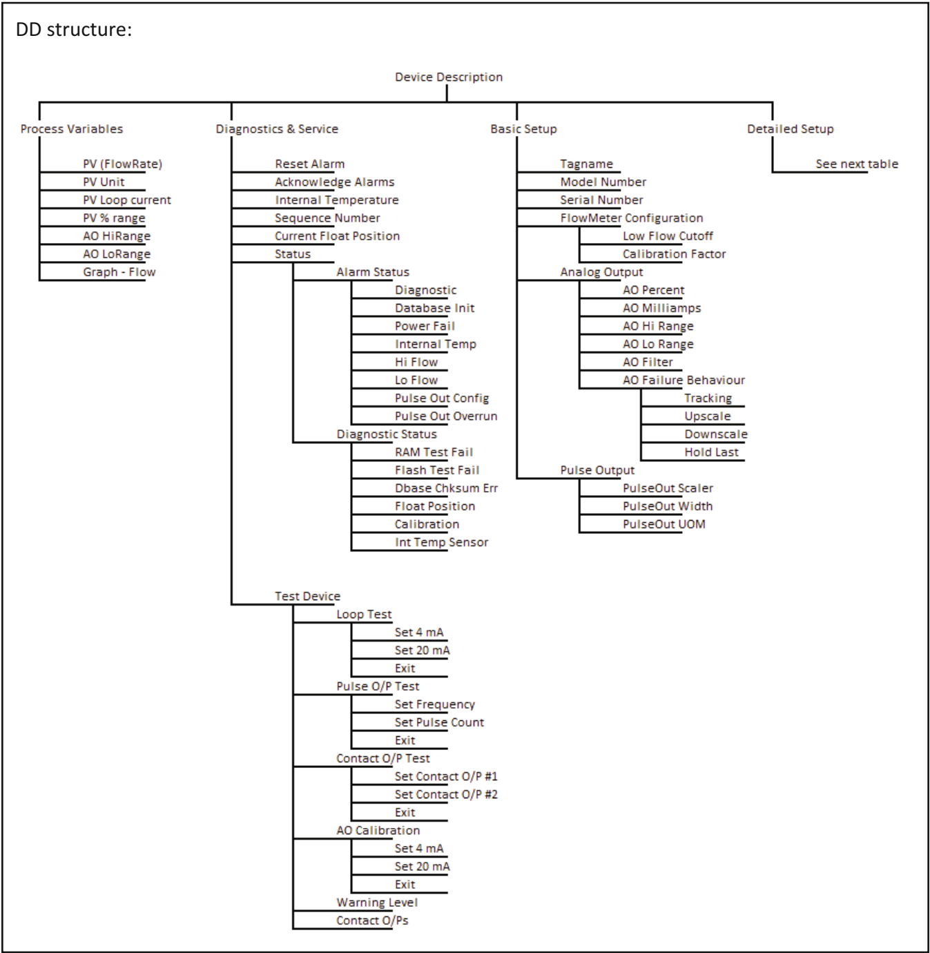
Figure 3-1 Model MT3809 Electronics Basic Setup Menu Tree
